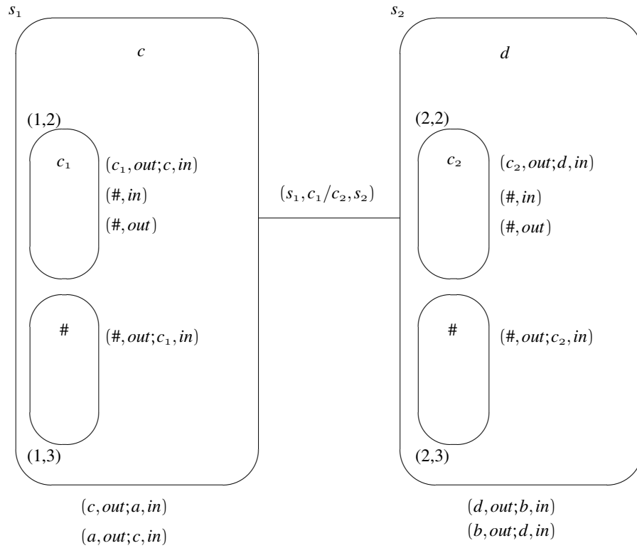
Figure 1: An example of a dP automaton
